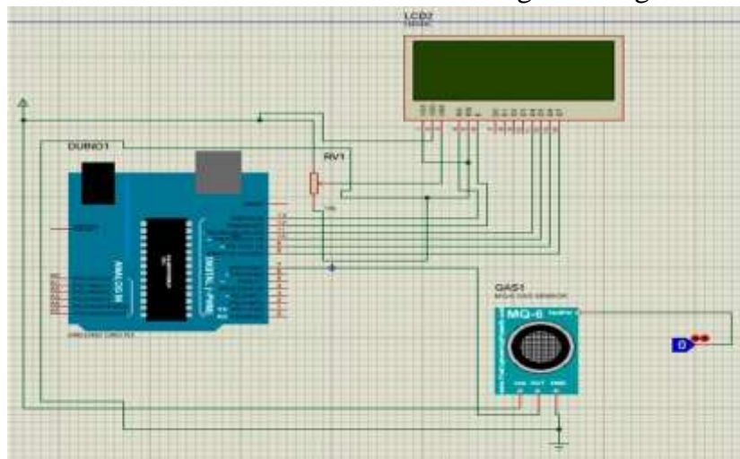
Figure 3. Circuit diagram that was designed using Proteus libraries.
