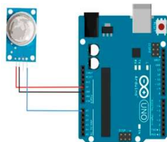
Figure 4. Circuit diagram of MQ-6 gas sensor connected with Arduino.
