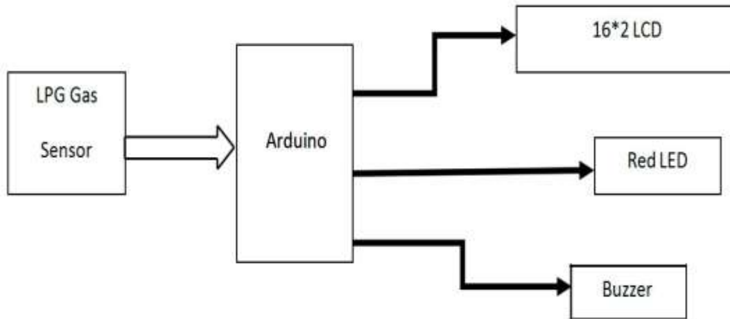
Figure 1. Block diagram of gas leakage detection and alert system.
