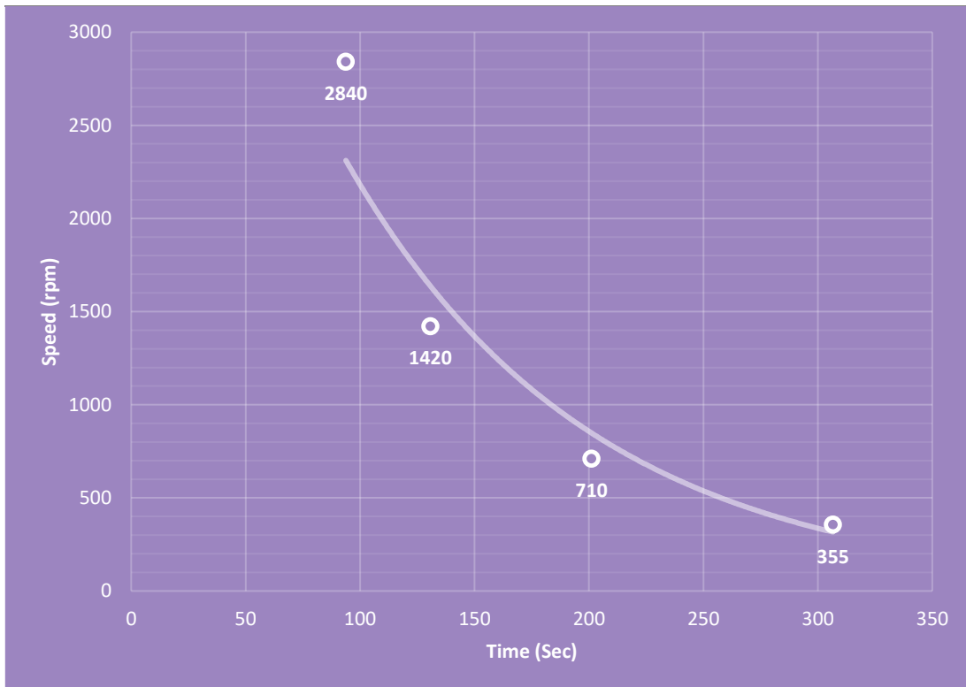
Figure 4: Graph of dehydration time of 3kg of spent grain against speed
