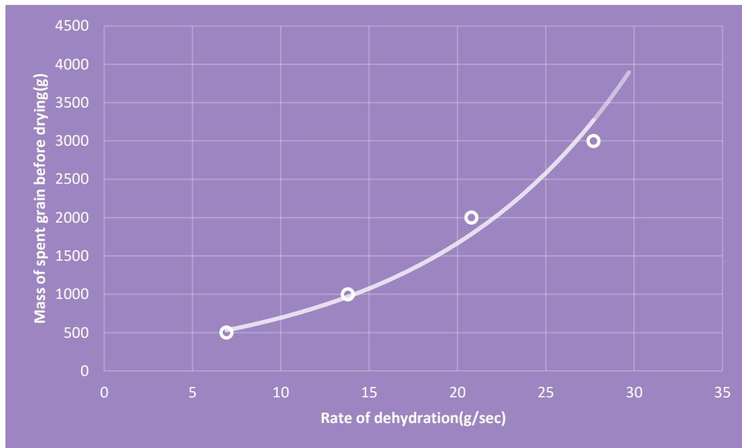
Figure 3: Graph of mass of spent grain against rate of dehydration at speed of 2840rpm for 30sec.
